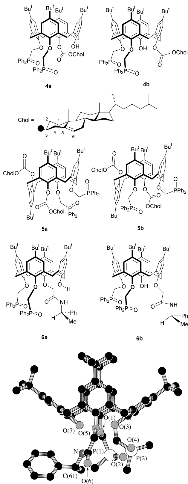
Fig. 1 Molecular structure of the chiral di(phosphine oxide) 6a (for clarity only the ipso carbon atoms of the PPh 2 groups are shown).
